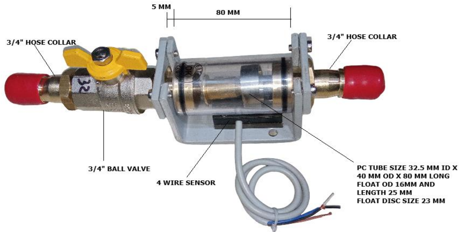
FLOW SWITCH 32 LPM WITH 3/4" BALL VALVE
